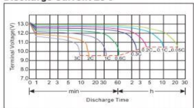
Discharge Current 25°C
